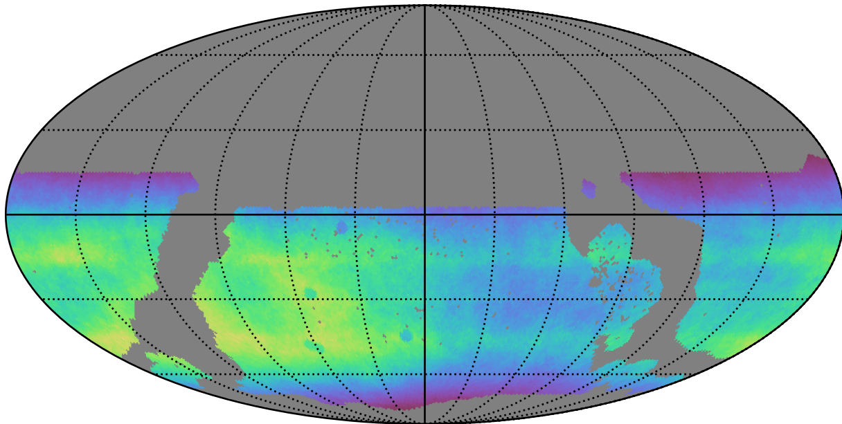
ddf_loaded_half_fl4_v3.4_10yrs WFD all bands: Normalized Teff
