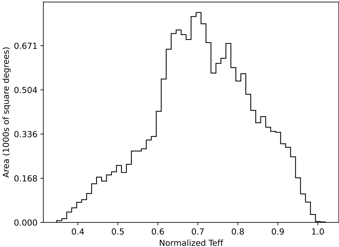
ddf_loaded_half_fl4_v3.4_10yrs WFD all bands: Normalized Teff
