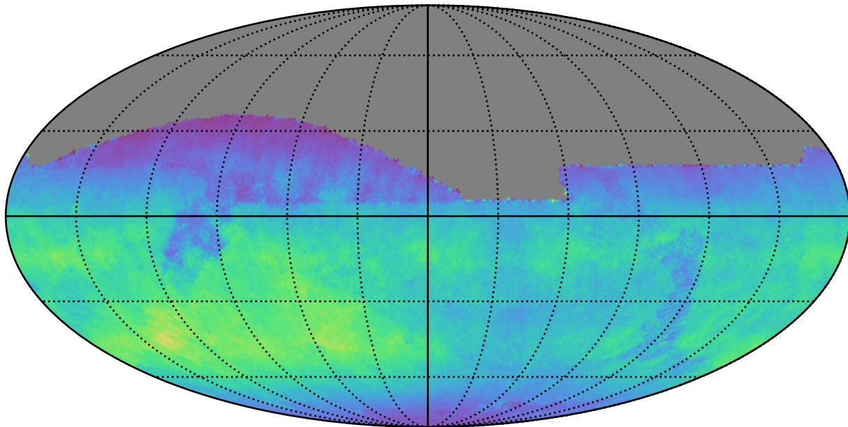
ddf_loaded_half_fl4_v3.4_10yrs All sky z band: Normalized Teff
