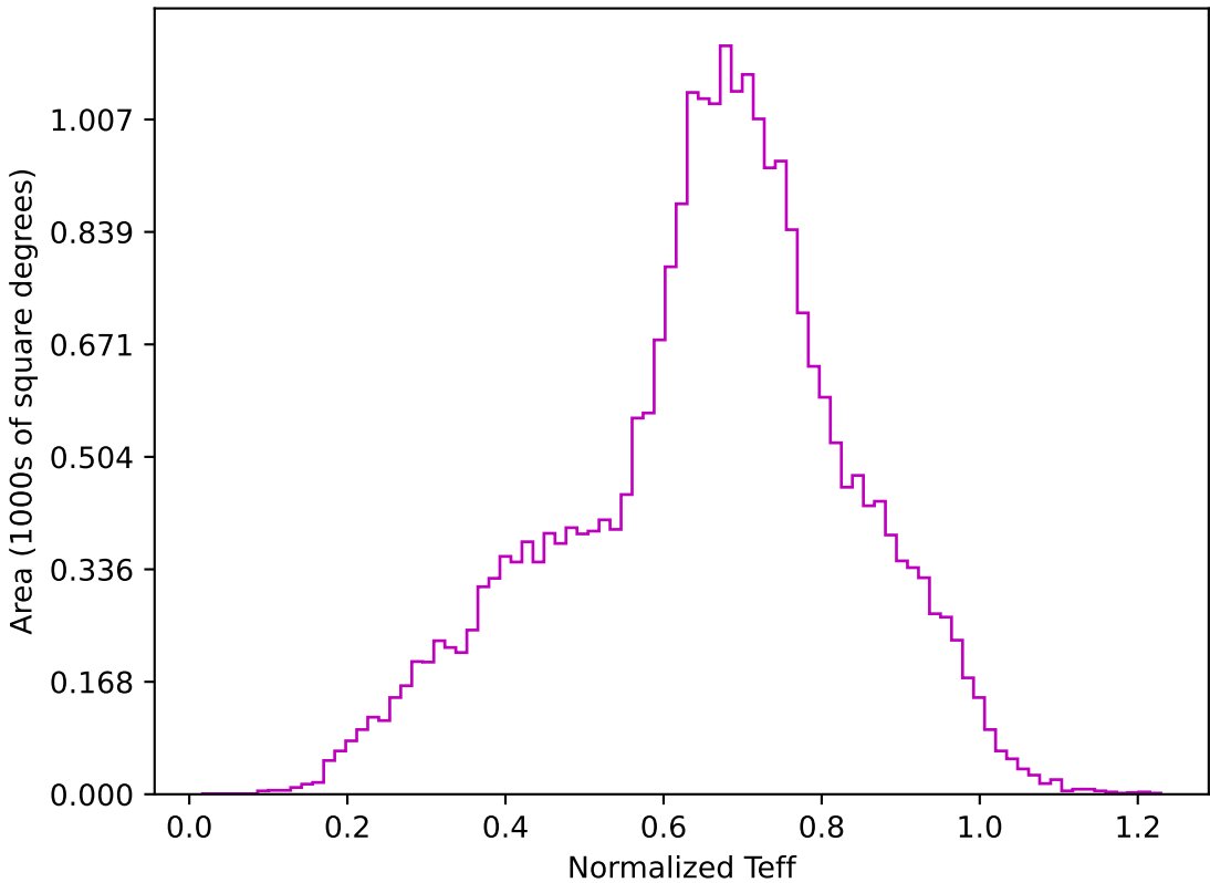
ddf_loaded_half_fl4_v3.4_10yrs All sky z band: Normalized Teff
