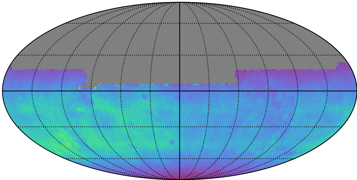
ddf_loaded_half_fl4_v3.4_10yrs All sky y band: Normalized Teff
