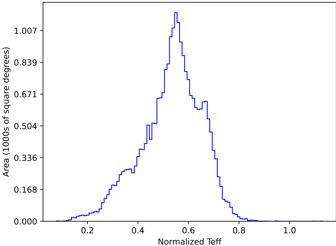
ddf_loaded_half_fl4_v3.4_10yrs All sky y band: Normalized Teff
