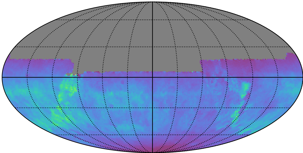
ddf_loaded_half_fl4_v3.4_10yrs All sky u band: Normalized Teff
