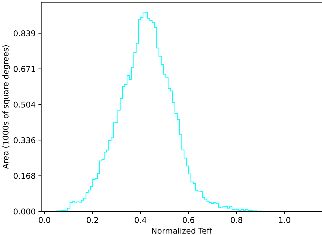
ddf_loaded_half_fl4_v3.4_10yrs All sky u band: Normalized Teff
