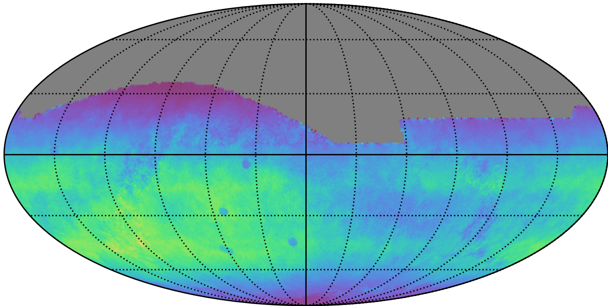
ddf_loaded_half_fl4_v3.4_10yrs All sky r band: Normalized Teff
