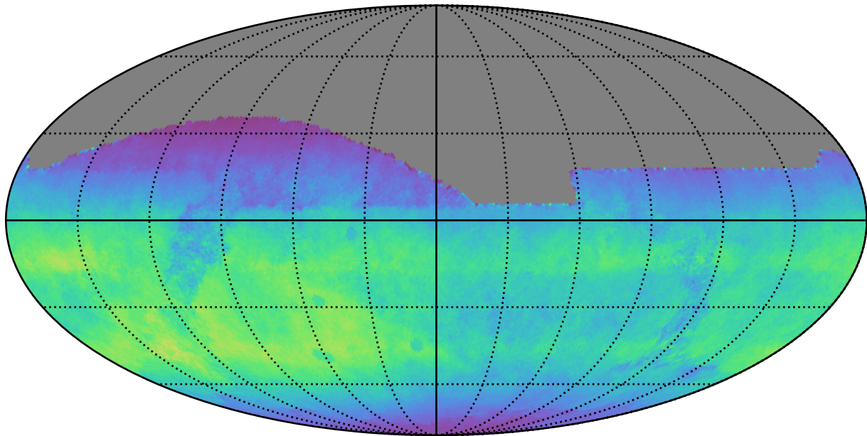
ddf_loaded_half_fl4_v3.4_10yrs All sky i band: Normalized Teff
