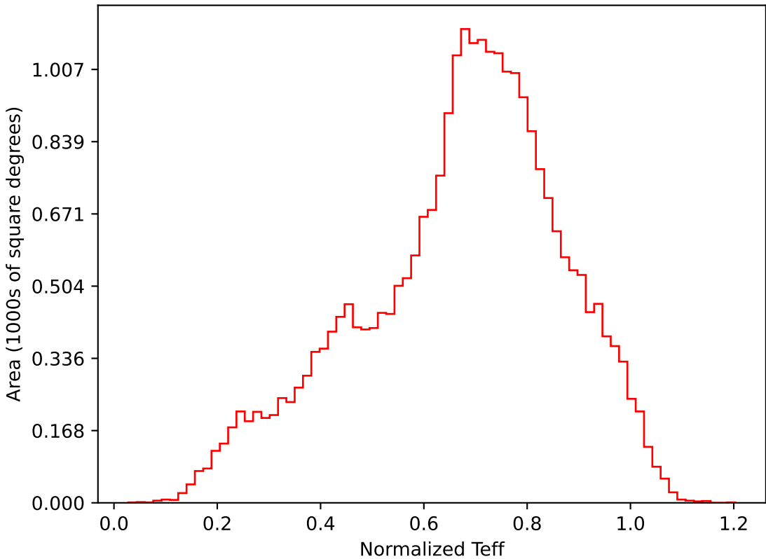
ddf_loaded_half_fl4_v3.4_10yrs All sky i band: Normalized Teff
