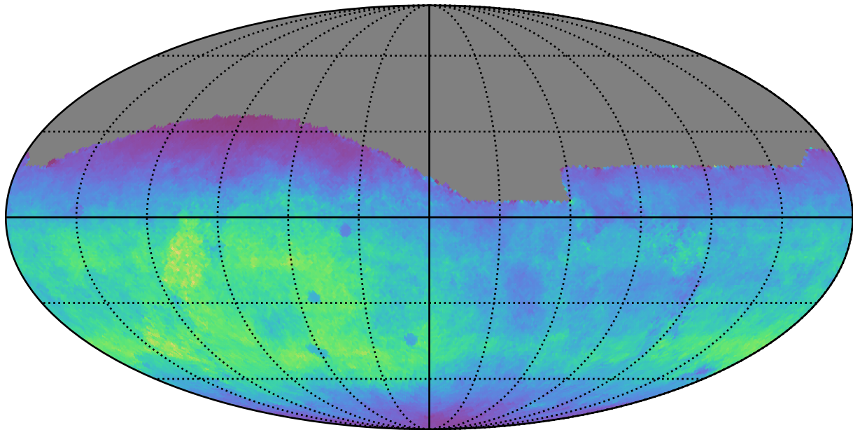
ddf_loaded_half_fl4_v3.4_10yrs All sky g band: Normalized Teff
