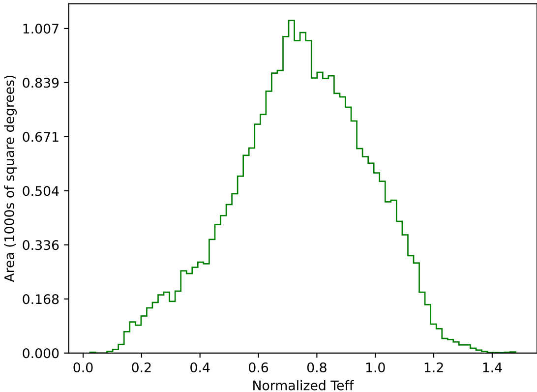
ddf_loaded_half_fl4_v3.4_10yrs All sky g band: Normalized Teff
