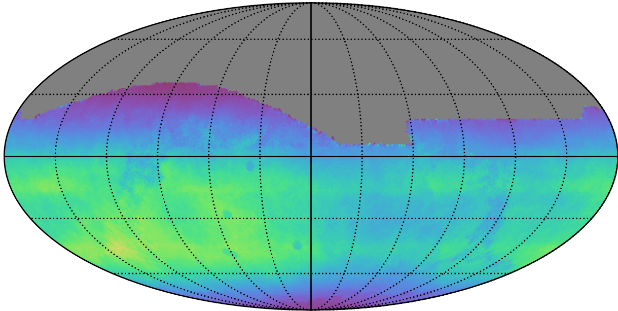
ddf_loaded_half_fl4_v3.4_10yrs All sky all bands: Normalized Teff
