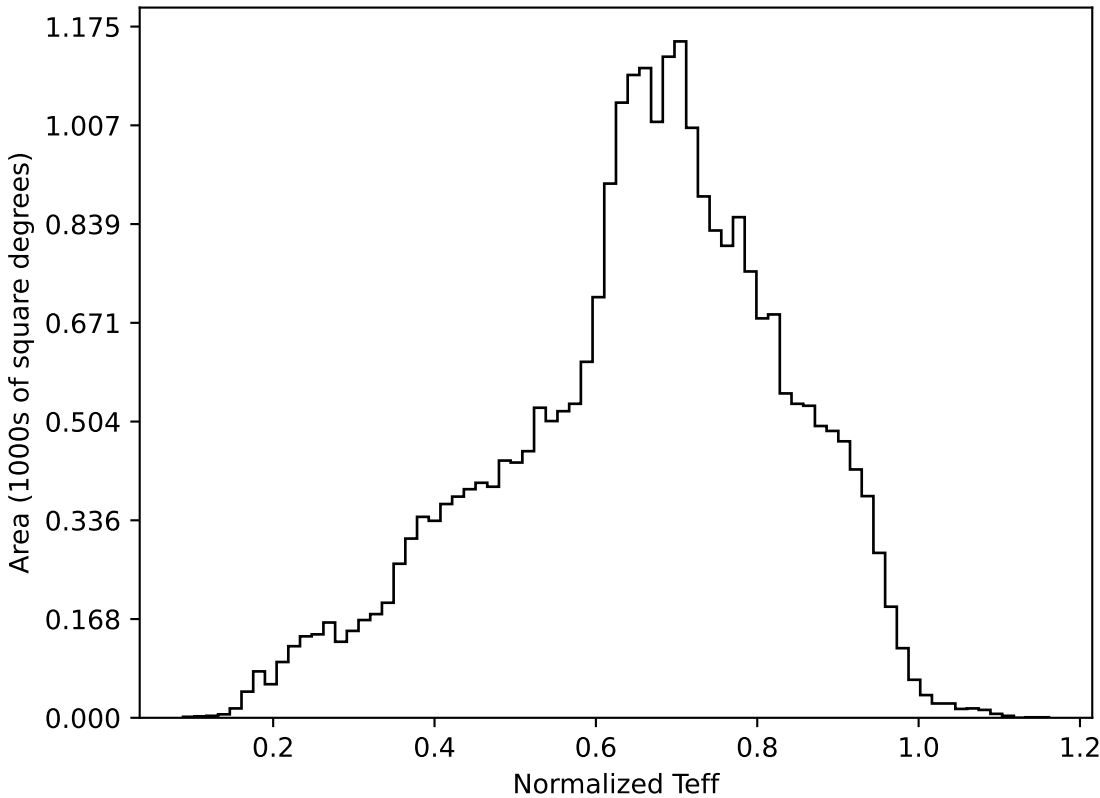
ddf_loaded_half_fl4_v3.4_10yrs All sky all bands: Normalized Teff
