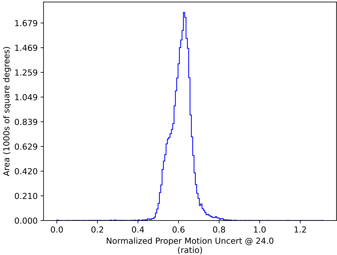
ddf_loaded_half_fl4_v3.4_10yrs All sky: Normalized Proper Motion Uncert @ 24.0
