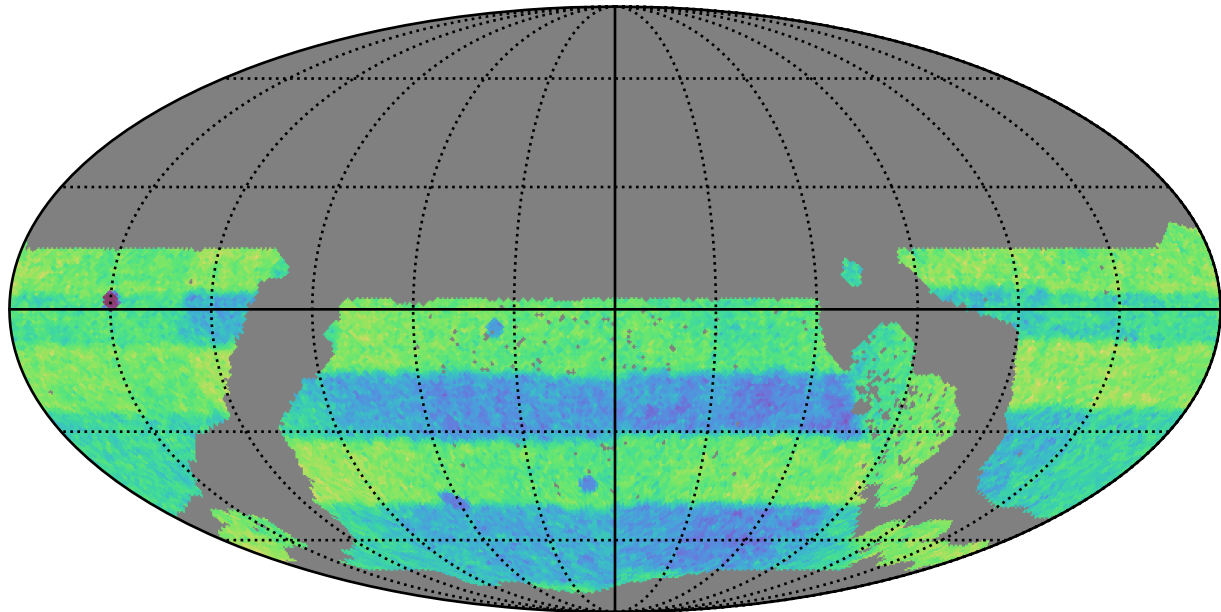
ddf_loaded_half_fl4_v3.4_10yrs WFD: Normalized Proper Motion Uncert @ 20.5
