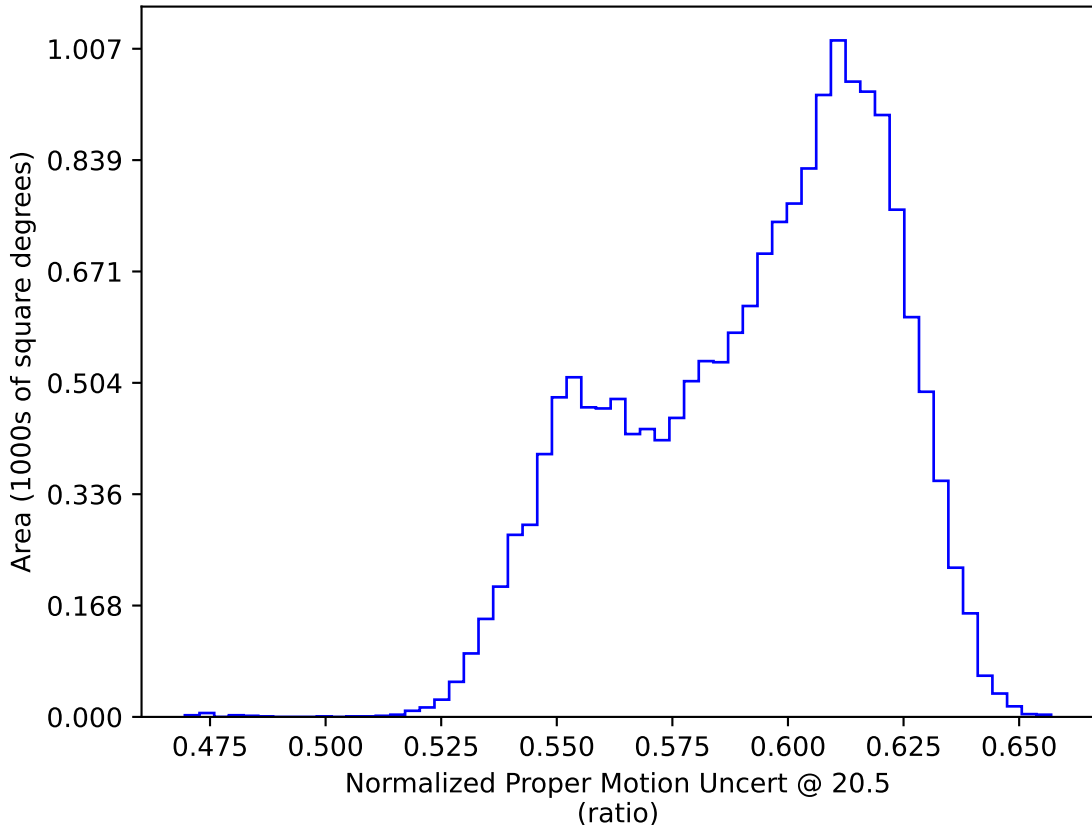
ddf_loaded_half_fl4_v3.4_10yrs WFD: Normalized Proper Motion Uncert @ 20.5
