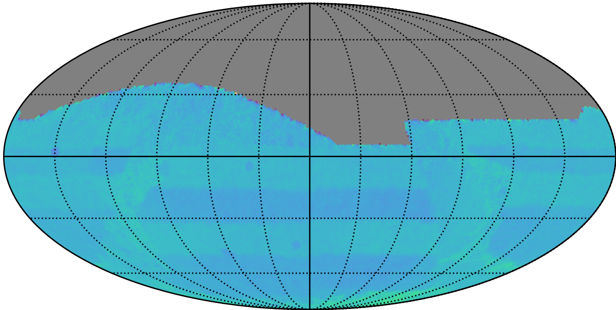
ddf_loaded_half_fl4_v3.4_10yrs All sky: Normalized Proper Motion Uncert @ 20.5
