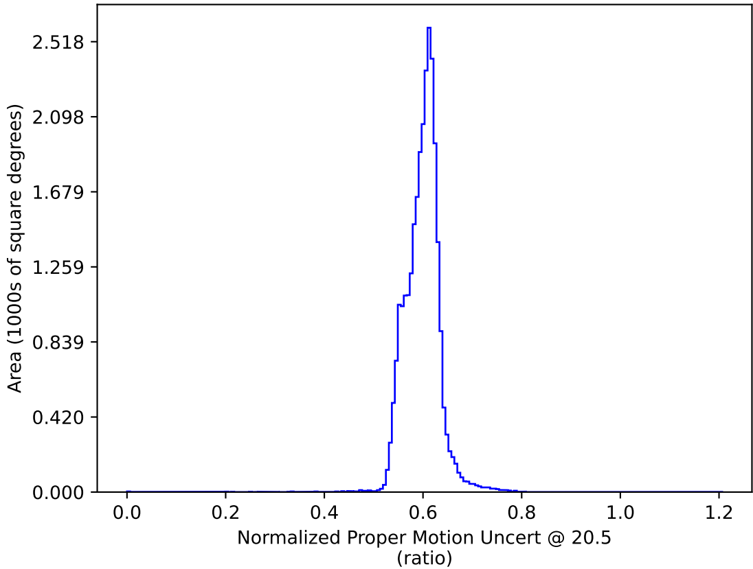
ddf_loaded_half_fl4_v3.4_10yrs All sky: Normalized Proper Motion Uncert @ 20.5
