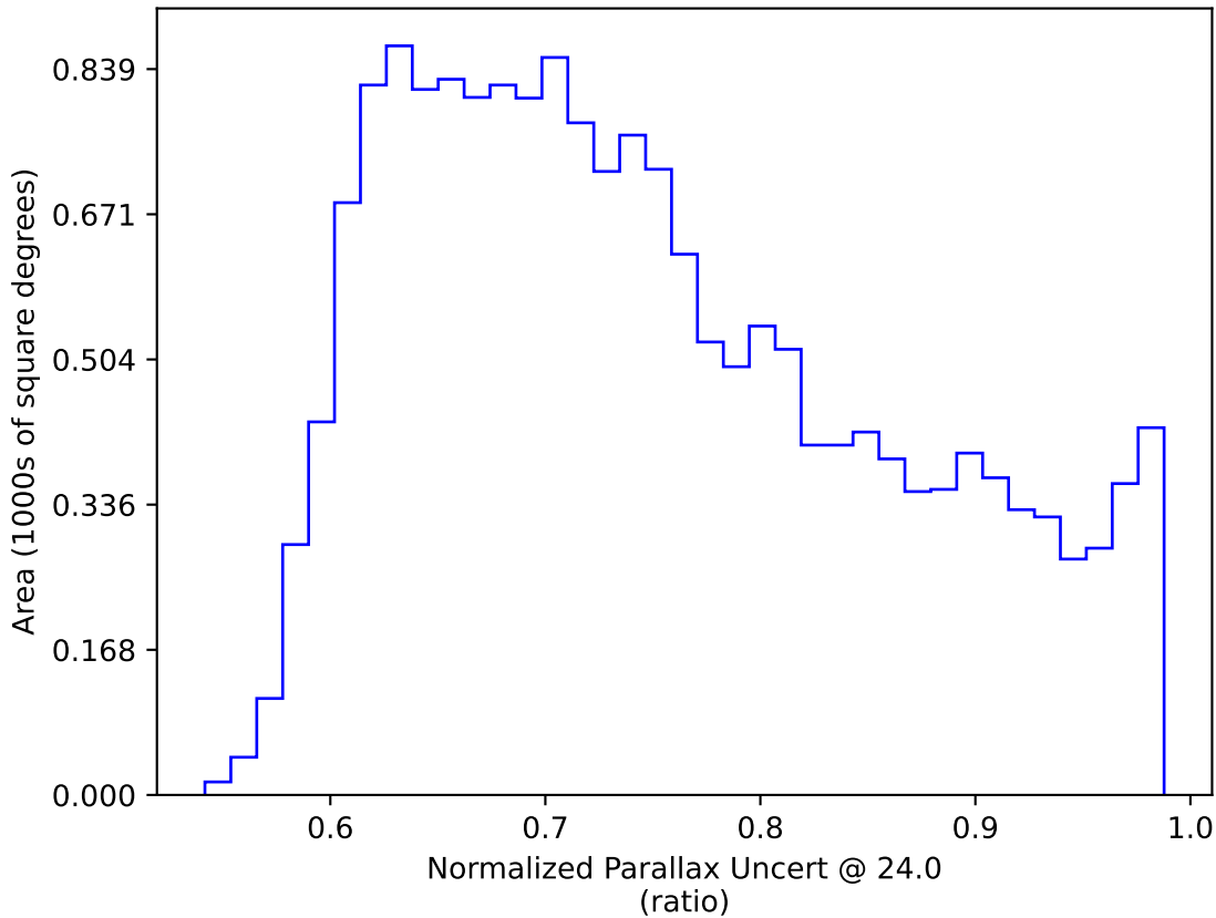
ddf_loaded_half_f14_v3.4_10yrs WFD: Normalized Parallax Uncert @ 24.0
