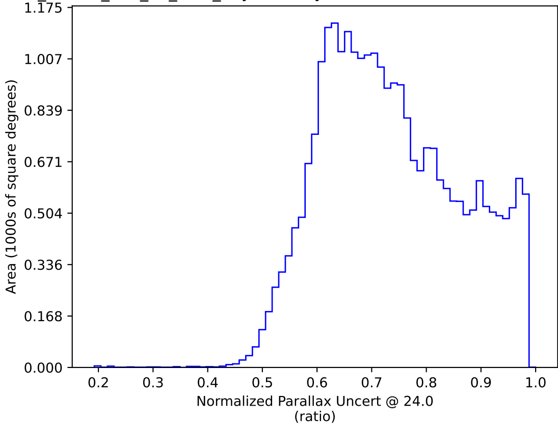
ddf_loaded_half_fl4_v3.4_10yrs All sky: Normalized Parallax Uncert @ 24.0
