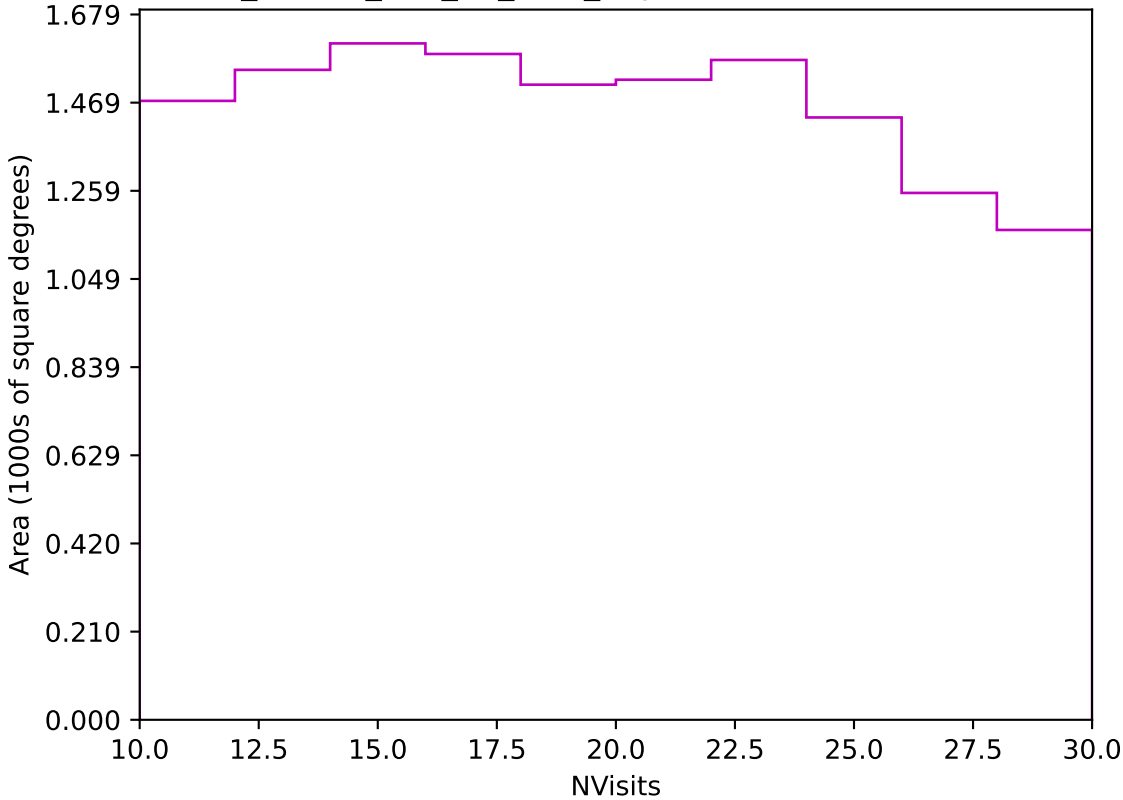
ddf_loaded_half_fl4_v3.4_10yrs Yr 3-4 z band: NVisits
