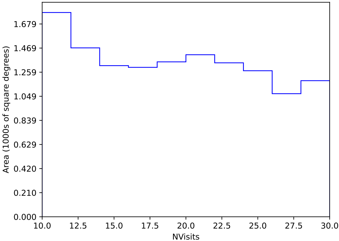
ddf_loaded_half_fi4_v3.4_10yrs Yr 3-4 y band: NVisits
