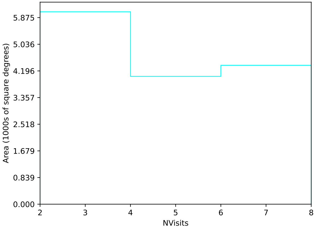
ddf_loaded_half_fl4_v3.4_10yrs Yr 3-4 u band: NVisits
