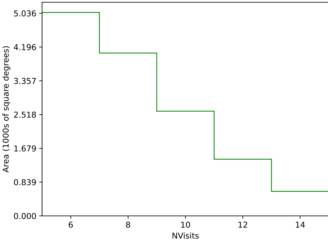
ddf_loaded_half_fl4_v3.4_10yrs Yr 3-4 g band: NVisits
