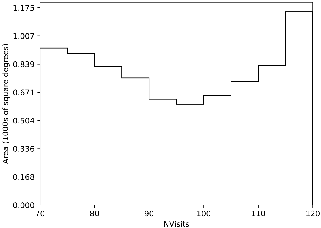
ddf_loaded_half_fl4_v3.4_10yrs Yr 3-4 all bands: NVisits
