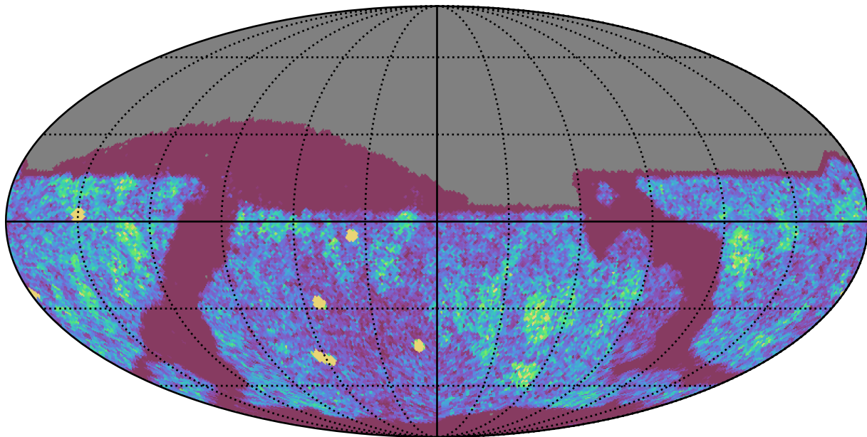
ddf_loaded_half_fl4_v3.4_10yrs Yr 1 z band: NVisits
