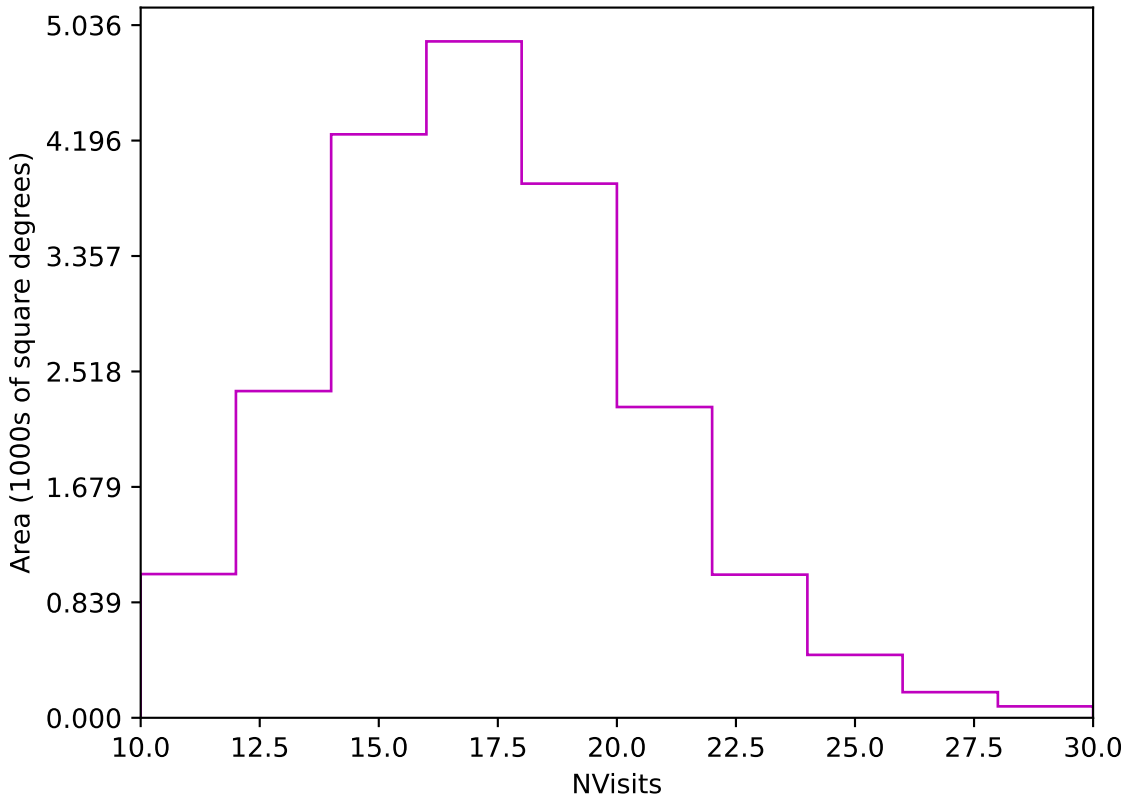
ddf_loaded_half_fl4_v3.4_10yrs Yr 1 z band: NVisits
