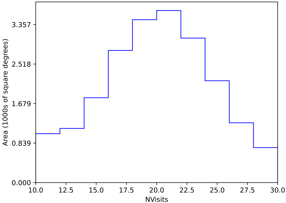
ddf_loaded_half_fl4_v3.4_10yrs Yr 1 y band: NVisits
