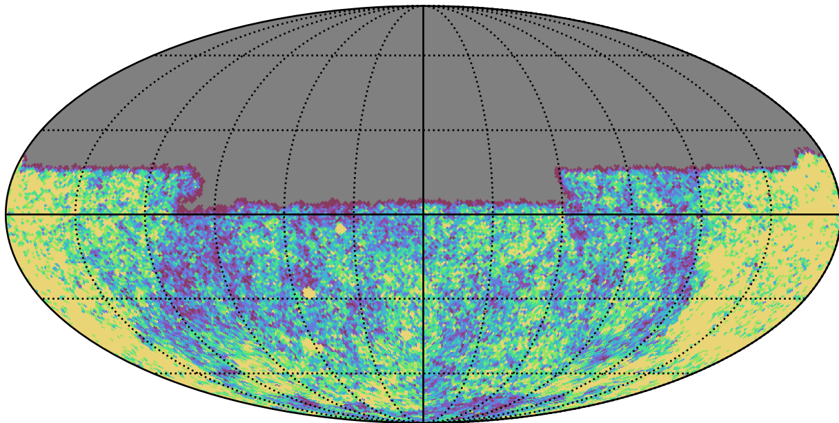
ddf_loaded_half_fl4_v3.4_10yrs Yr 1 u band: NVisits
