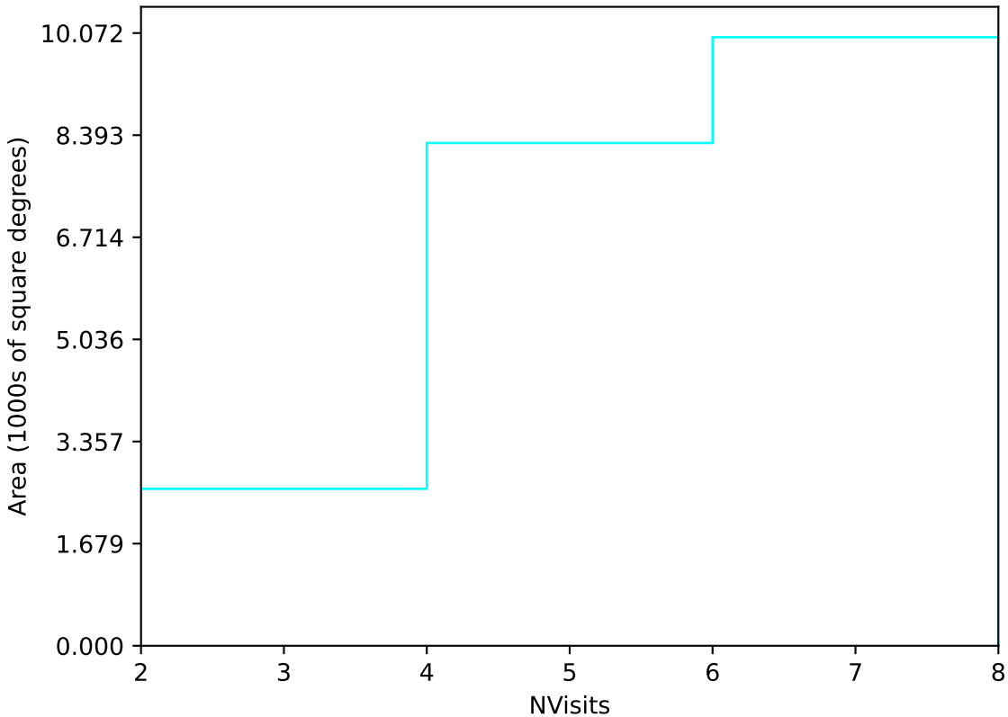
ddf_loaded_half_fl4_v3.4_10yrs Yr 1 u band: NVisits
