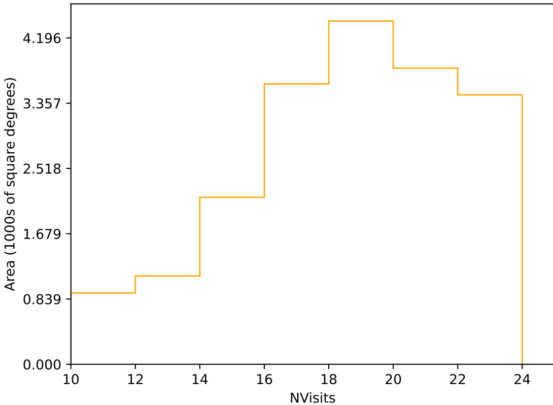
ddf_loaded_half_fl4_v3.4_10yrs Yr 1 r band: NVisits
