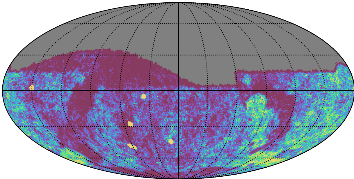
ddf_loaded_half_fl4_v3.4_10yrs Yr 1 g band: NVisits
