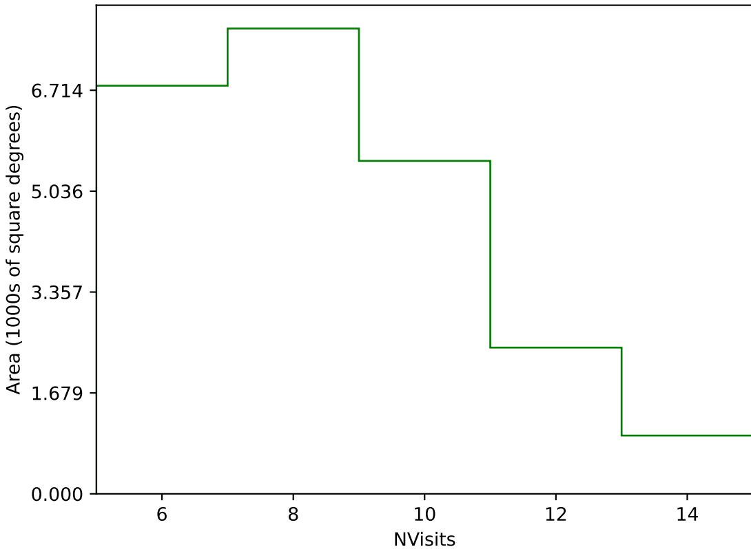
ddf_loaded_half_fl4_v3.4_10yrs Yr 1 g band: NVisits
