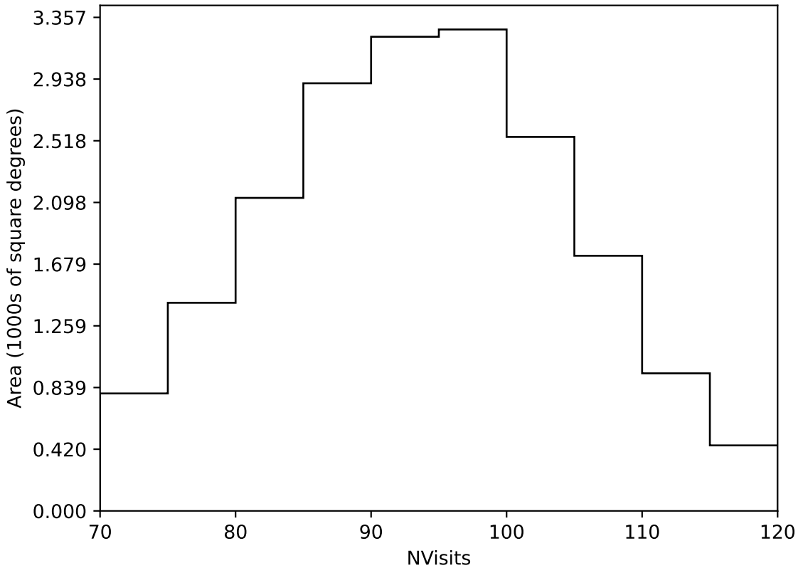
ddf_loaded_half_fl4_v3.4_10yrs Yr 1 all bands: NVisits
