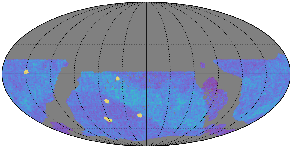
ddf_loaded_half_fl4_v3.4_10yrs WFD z band: NVisits
