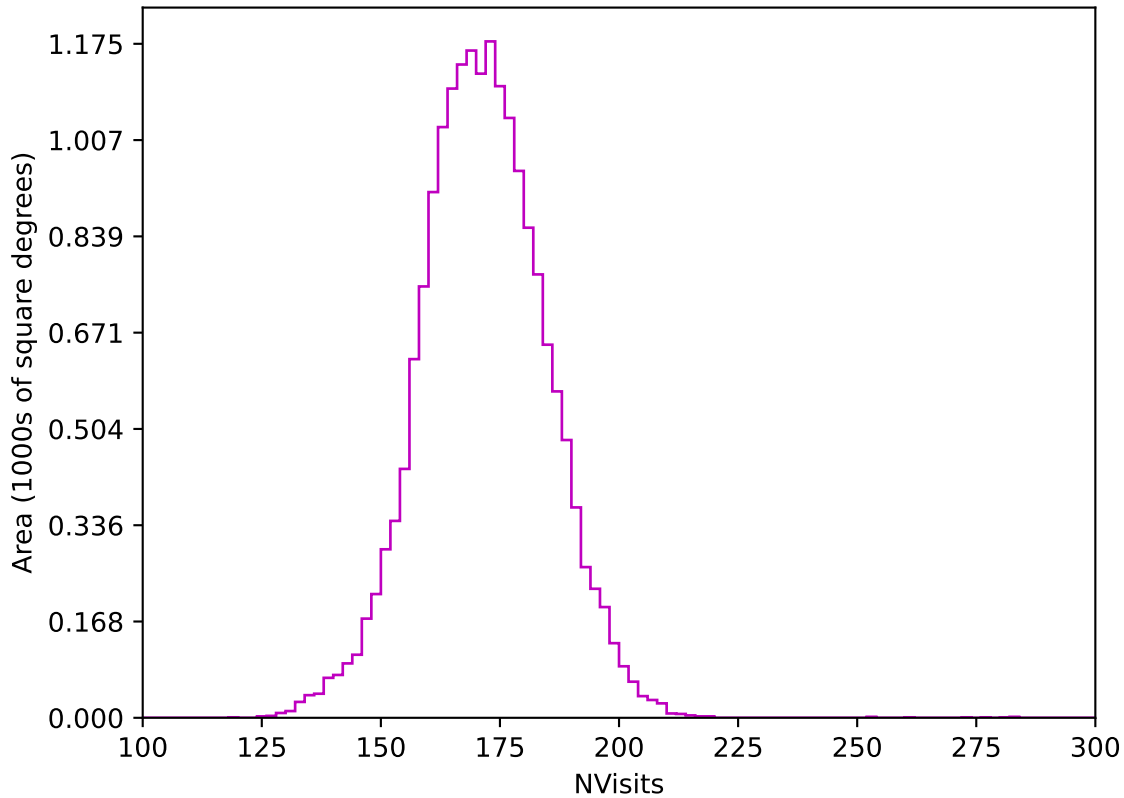
ddf_loaded_half_fl4_v3.4_10yrs WFD z band: NVisits
