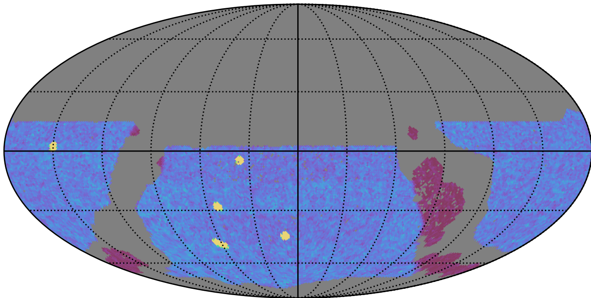
ddf_loaded_half_fl4_v3.4_10yrs WFD y band: NVisits
