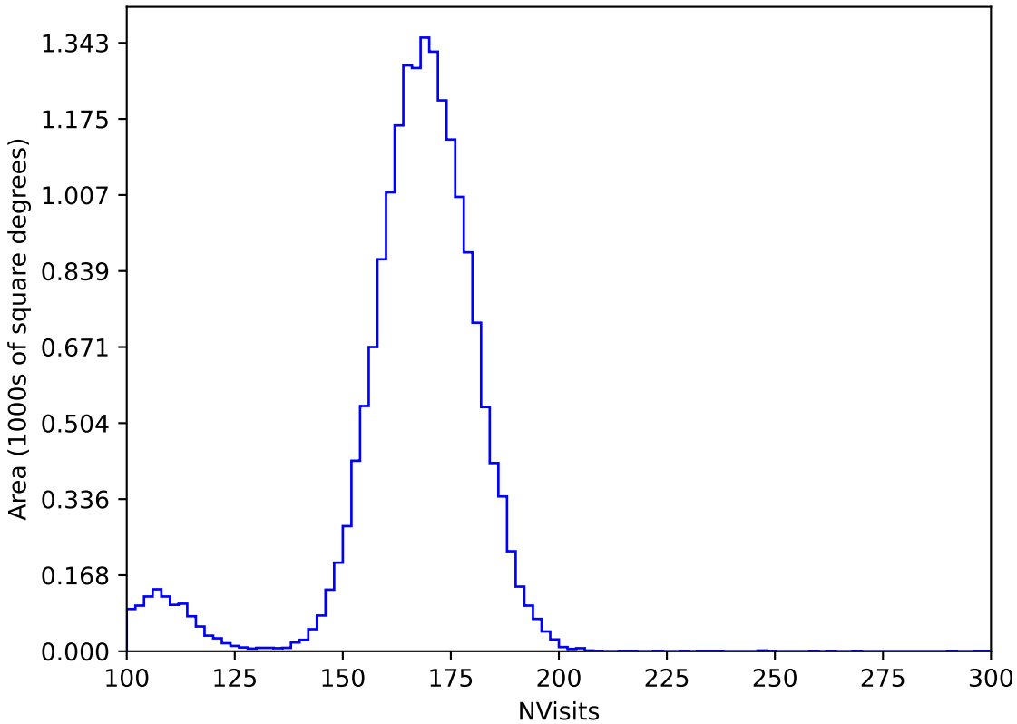
ddf_loaded_half_fl4_v3.4_10yrs WFD y band: NVisits
