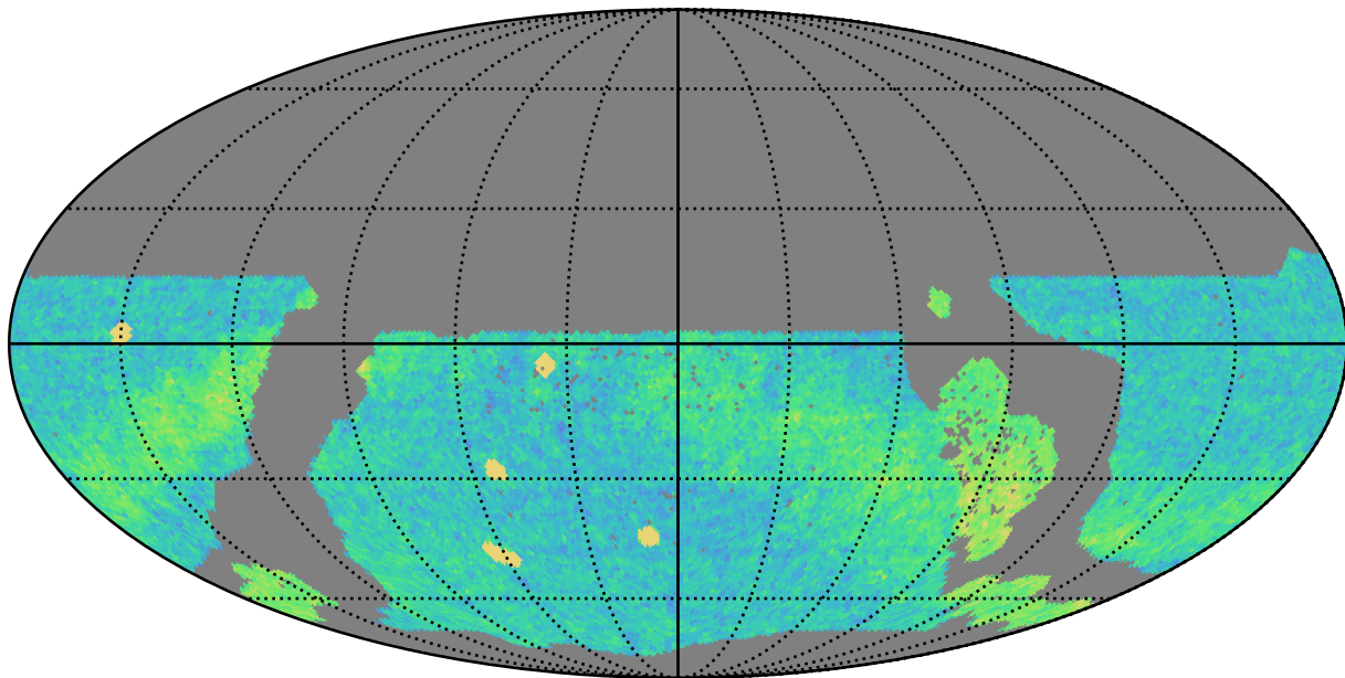
ddf_loaded_half_fl4_v3.4_10yrs WFD r band: NVisits
