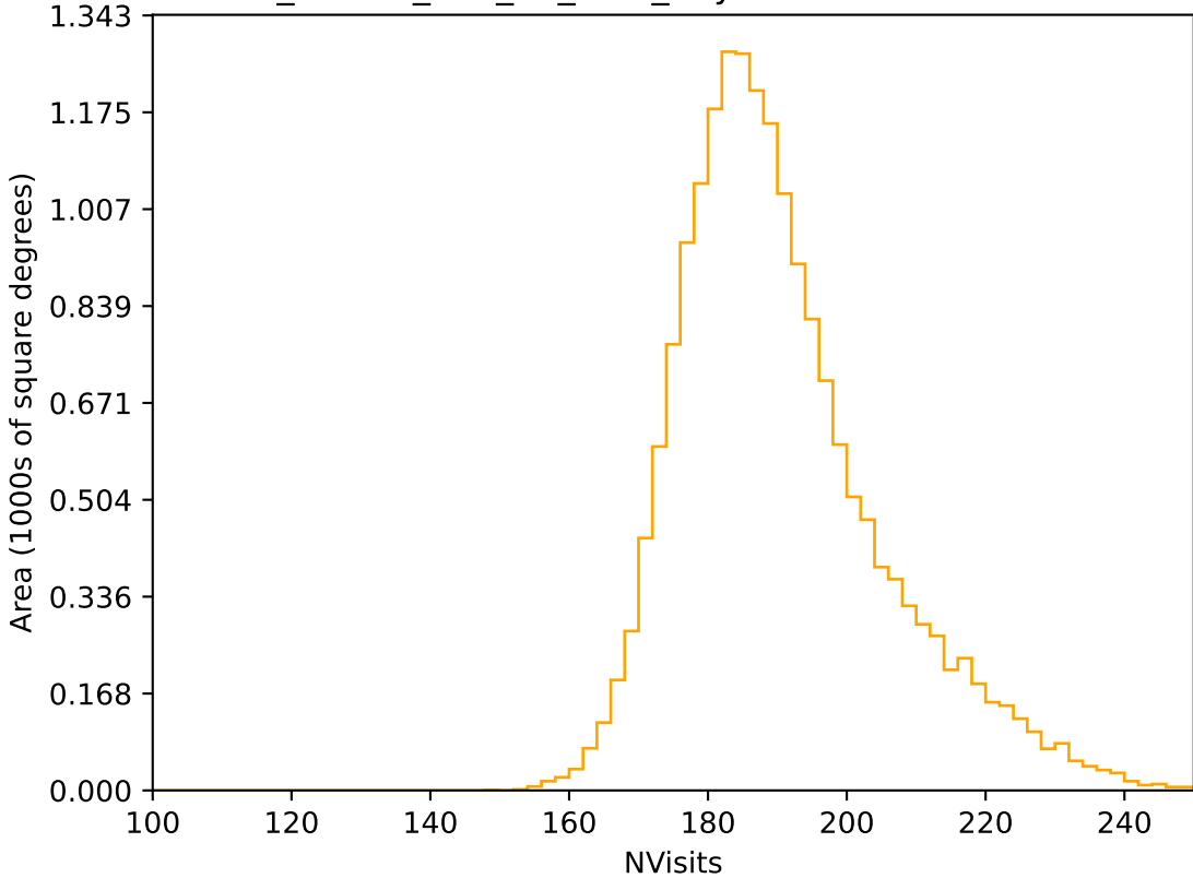
ddf_loaded_half_fl4_v3.4_10yrs WFD r band: NVisits
