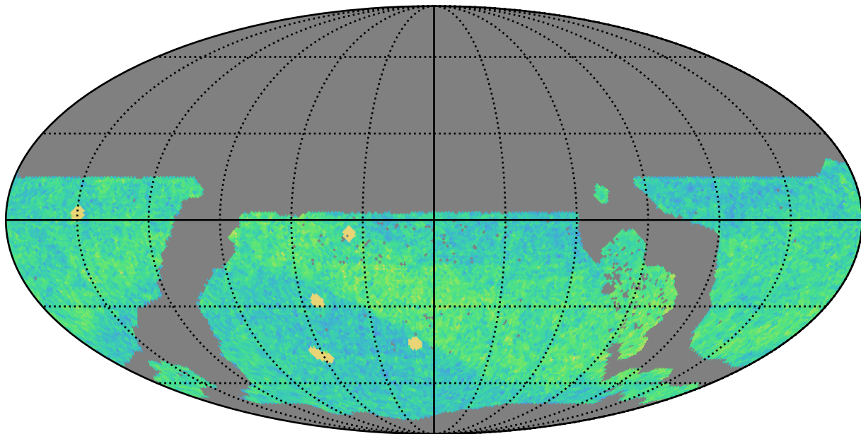
ddf_loaded_half_fl4_v3.4_10yrs WFD i band: NVisits
