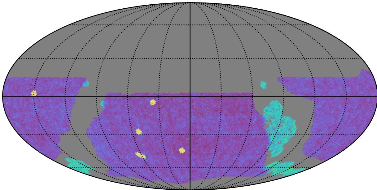
ddf_loaded_half_fl4_v3.4_10yrs WFD g band: NVisits
