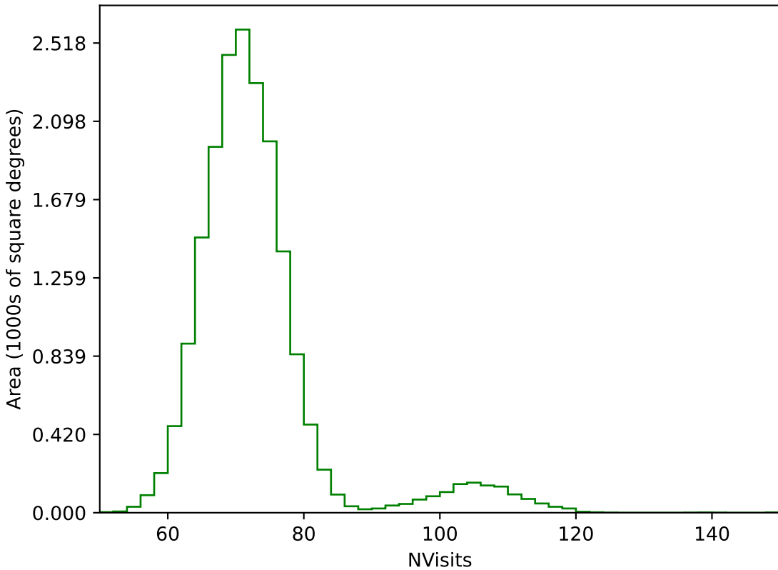
ddf_loaded_half_fl4_v3.4_10yrs WFD g band: NVisits
