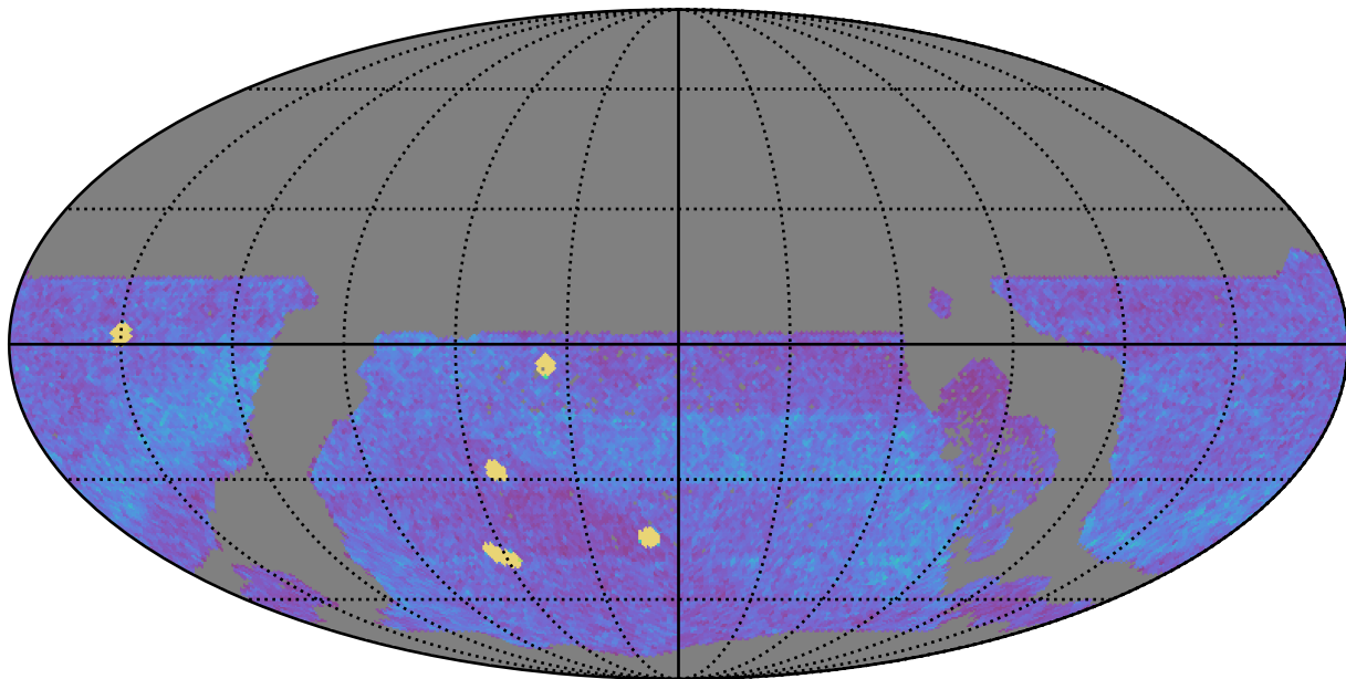
ddf_loaded_half_fl4_v3.4_10yrs WFD all bands: NVisits
