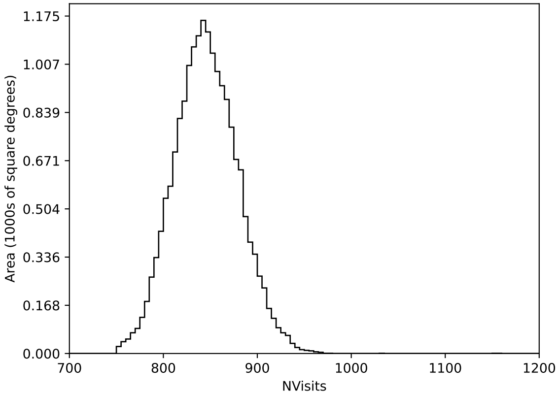
ddf_loaded_half_fl4_v3.4_10yrs WFD all bands: NVisits
