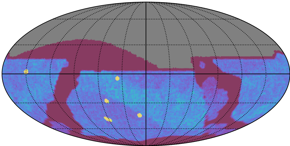
ddf_loaded_half_fl4_v3.4_10yrs All sky z band: NVisits
