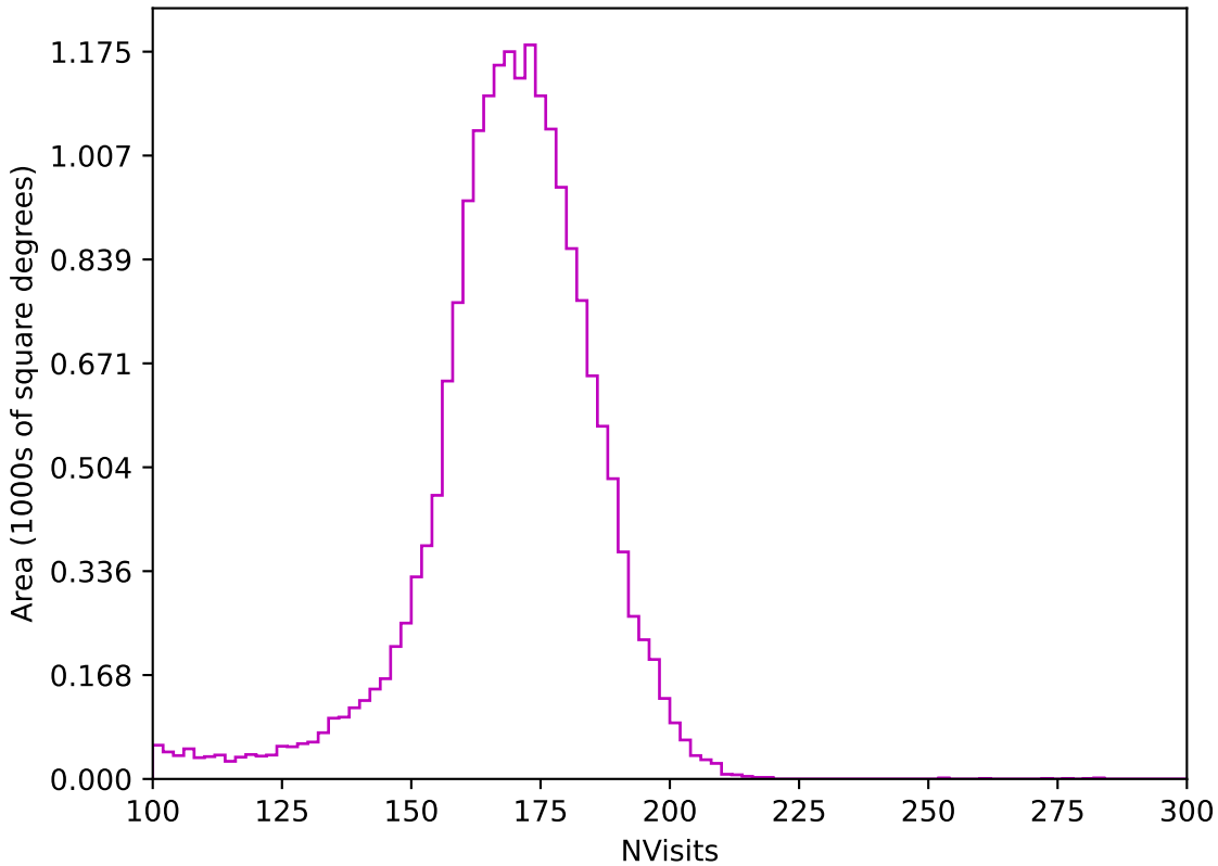
ddf_loaded_half_fl4_v3.4_10yrs All sky z band: NVisits
