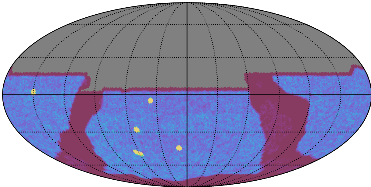
ddf_loaded_half_fl4_v3.4_10yrs All sky y band: NVisits
